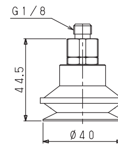
2 bellows suction cups PBG-40-N/S
