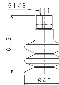
3 bellows suction cups PCG-40-N/S
