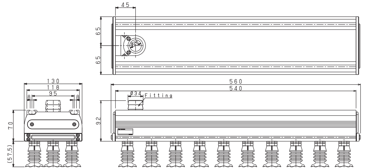
L560 type (With PMG-40 suction cups)
