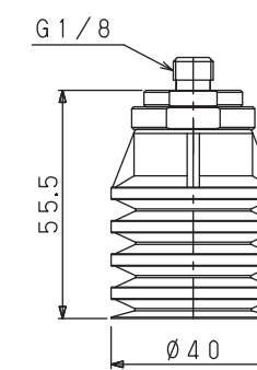
Multiple bellows suction cups PLG-40-S4/S5
