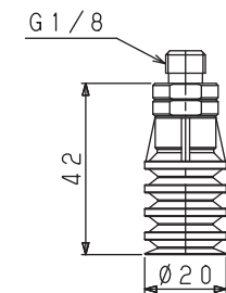
Multiple bellows suction cups PLG-20-S4/S5
