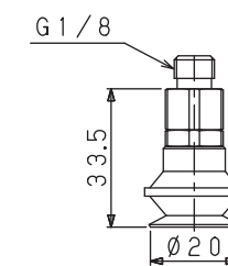
2 bellows suction cups PBG-20-N/S
