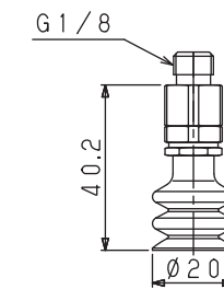
3 bellows suction cups PCG-20-N/S
