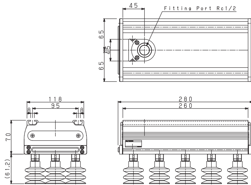
L280 type (With PCG-40 suction cups)
