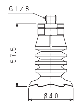
Star shaped multiple bellows suction cups PMG-40L-S4/S5
