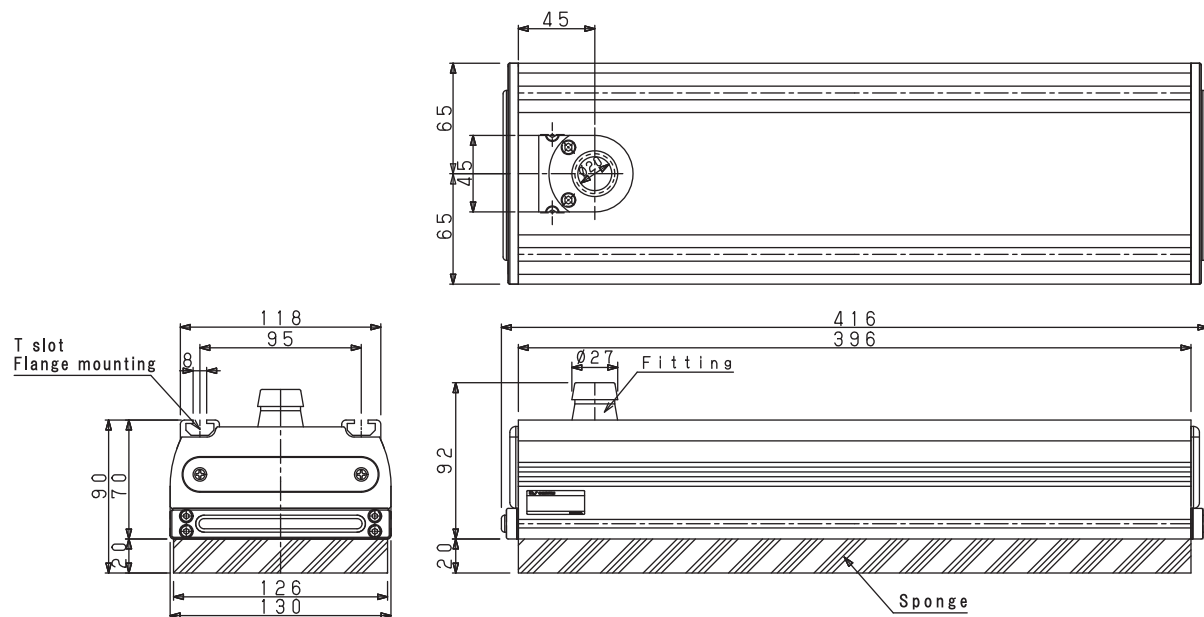
L416 type (With sponge pad)
