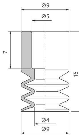
PCG-10
