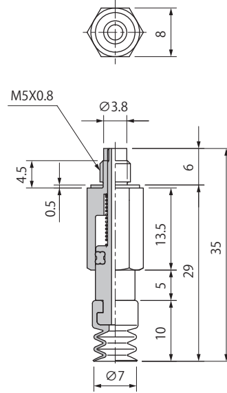
PSS-L5-PCG-7
