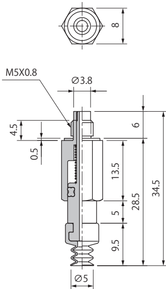
PSS-L5-PCG-5
