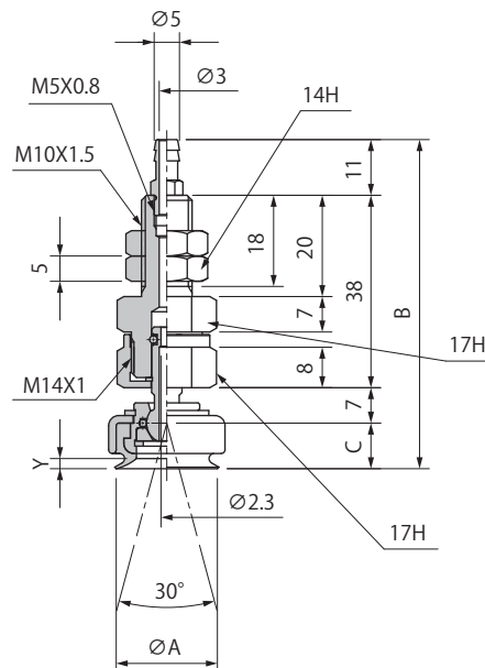
Top Port PUTKB-20 / 25 / 30 / 35
