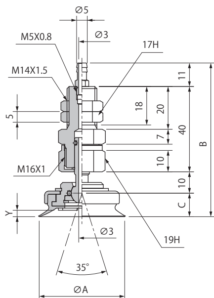
Top Port PUTKB-40 / 50
