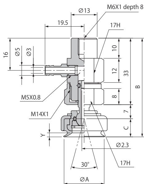
Side Port PUYKB-20 / 25 / 30 / 35
