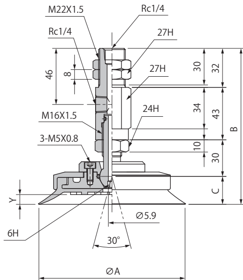
Top Port PUTKB-120 / 150
