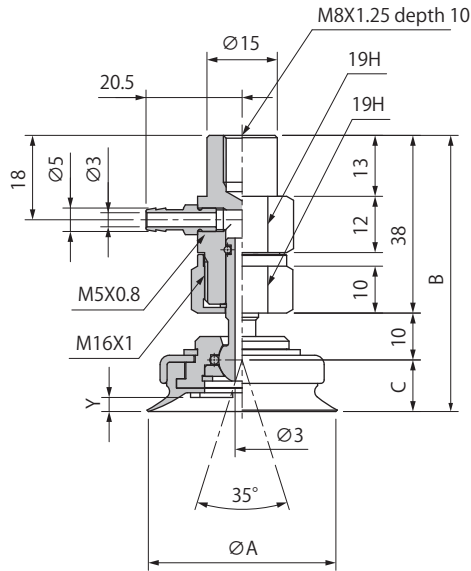
Side Port PUYKB-40 / 50
