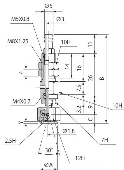
Top Port PUTKB-10 / 15
